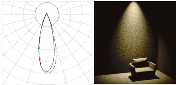
30° BEAM ANGLE
