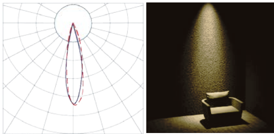
20° BEAM ANGLE
